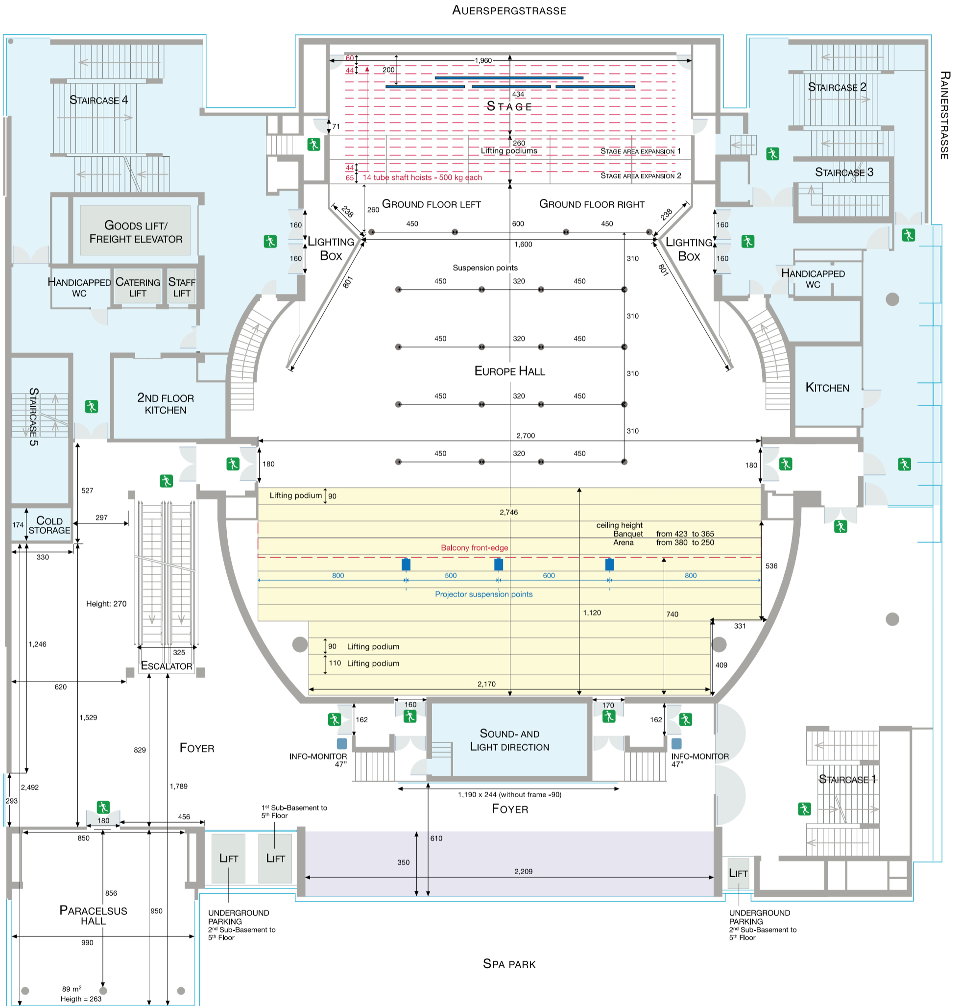
CAPTION 240 Length specifications in centimetres — Mobile walls — Fixed walls - - - Tube shaft hoist ■ Lifting podium ■ Closed area
